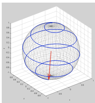
\omega = \omega_0
