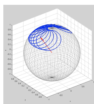
\omega = \omega_0
