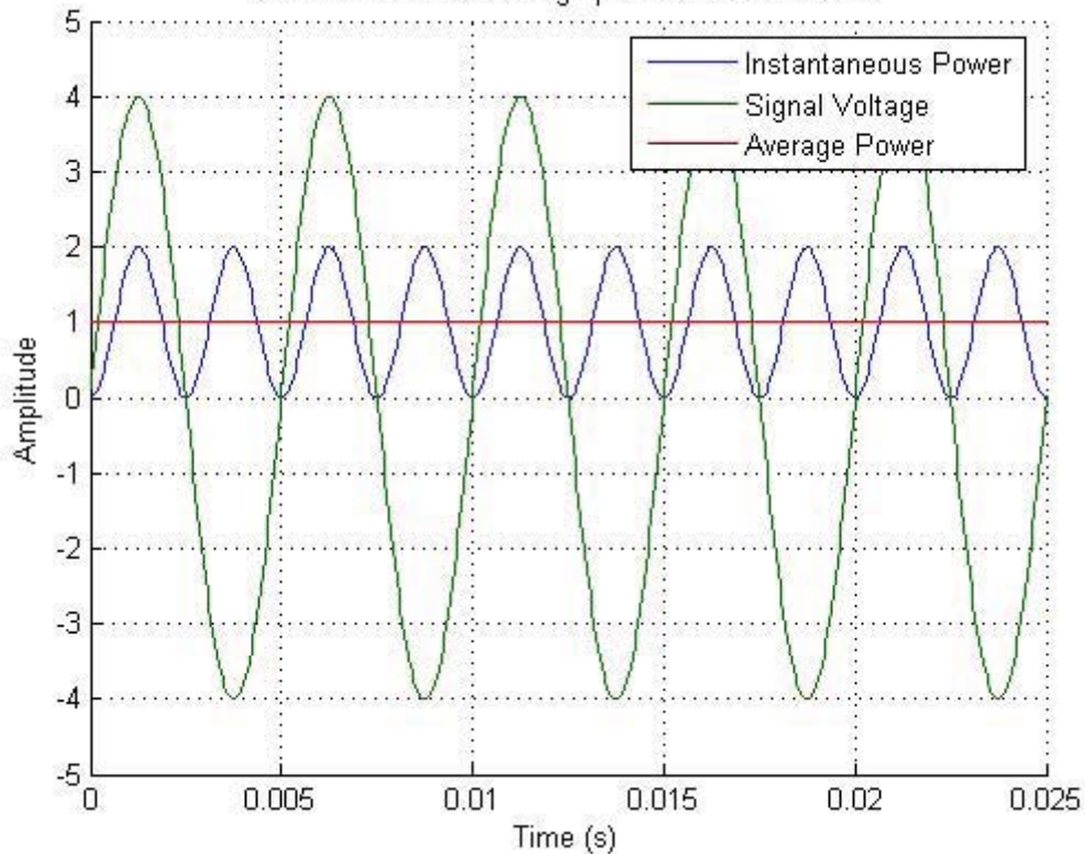
Instantaneous vs. average power into 8 ohm load
