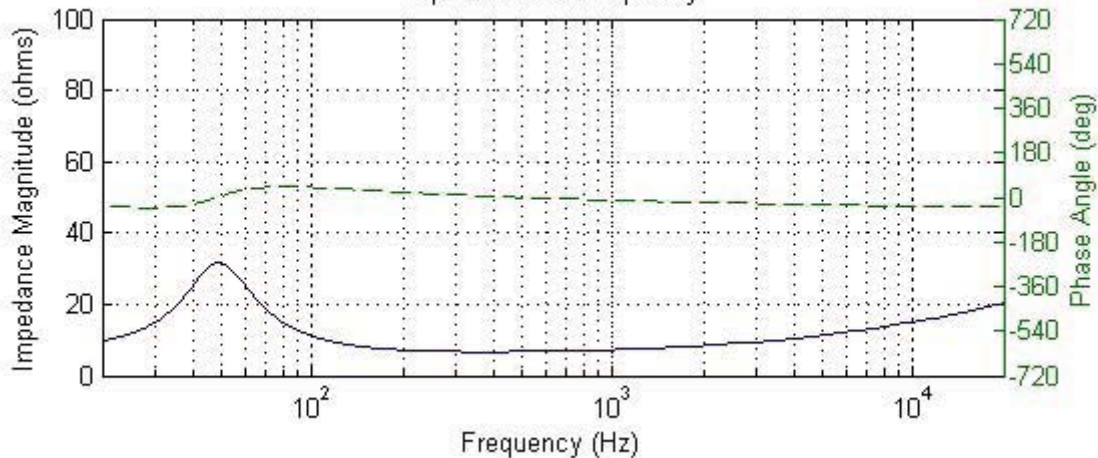
Impedance vs. Frequency
